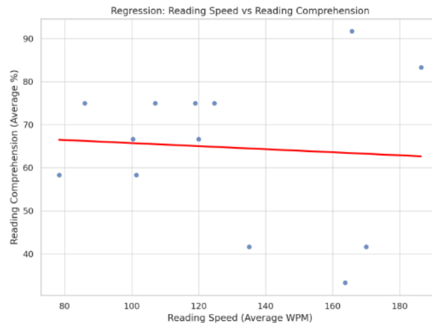
Figure 1. The regression plot
